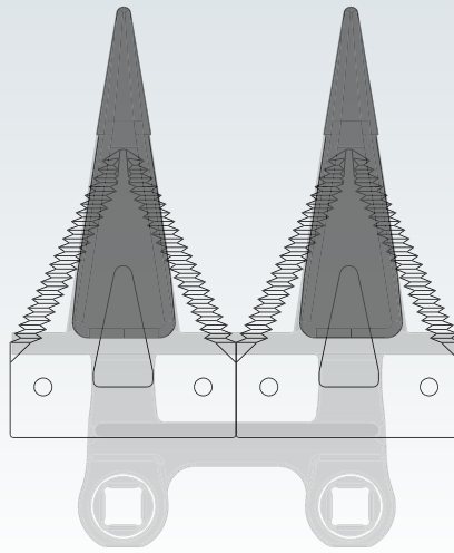
ClearCut™ Pointed Knife Guards
